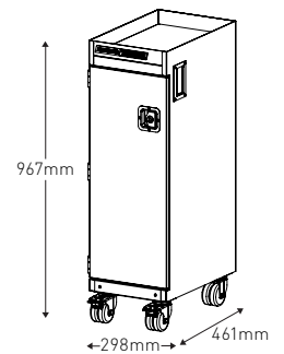
MOBILE PARTS TROLLEY 6 TRAY 300MM K7368
