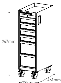
MOBILE SERVICE TROLLEY 6 DRAWER 300MM K7369
